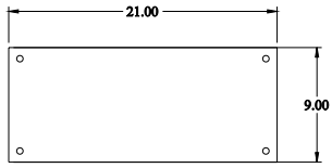
INNER PANEL
