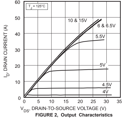
FIGURE 2, Output Characteristics
