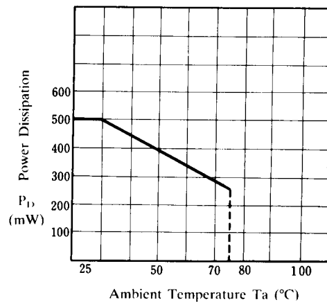
NJM2930L (TO-92)
