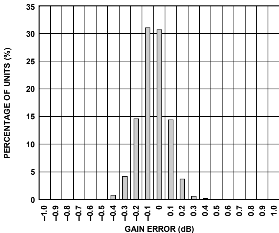
Figure 11. Gain Error Histogram, V_{GAIN} = 0 V
