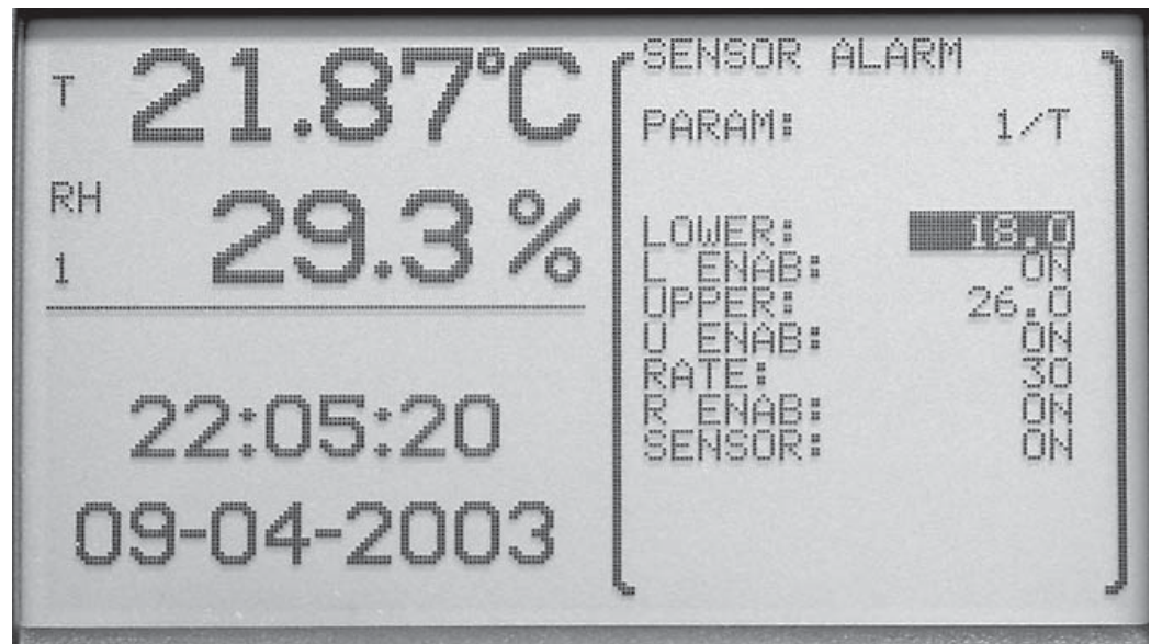
Figure 36 Sensor Alarm
