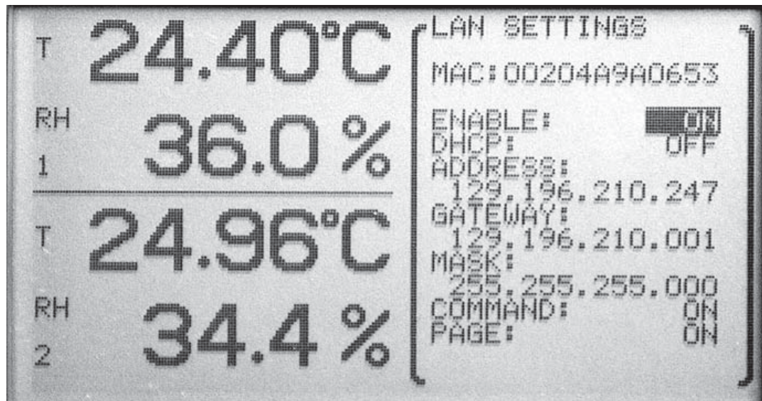
Figure 45 Lan Settings
