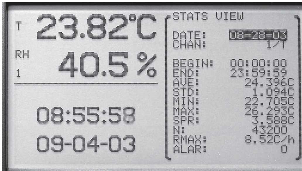
Figure 30 Stats View
