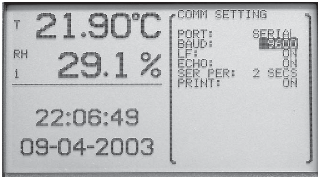
Figure 42 Comm Setting
