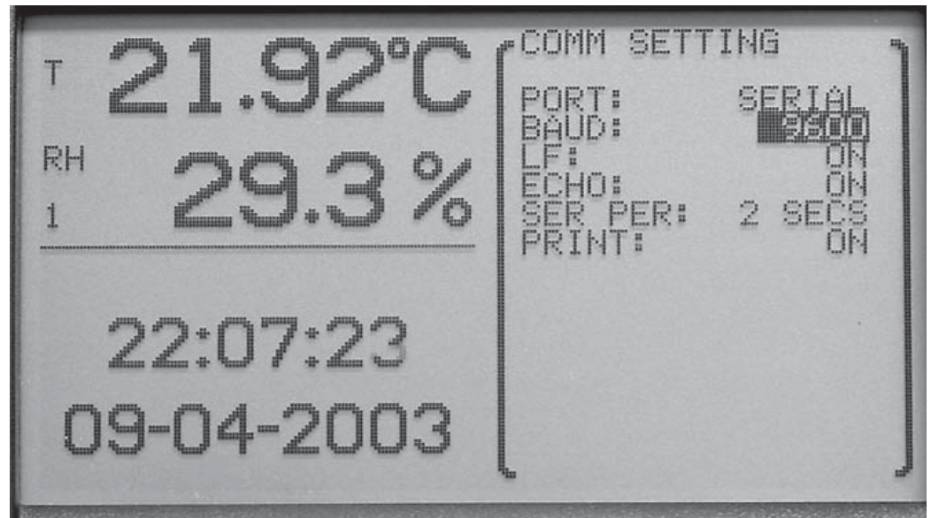
Figure 43 Serial
