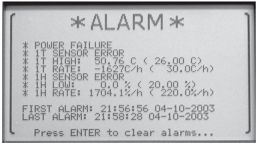
Figure 38 Alarm View
