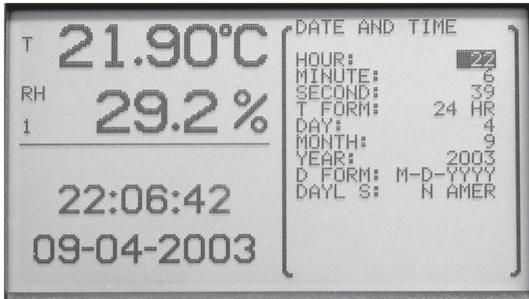
Figure 41 Date Time
