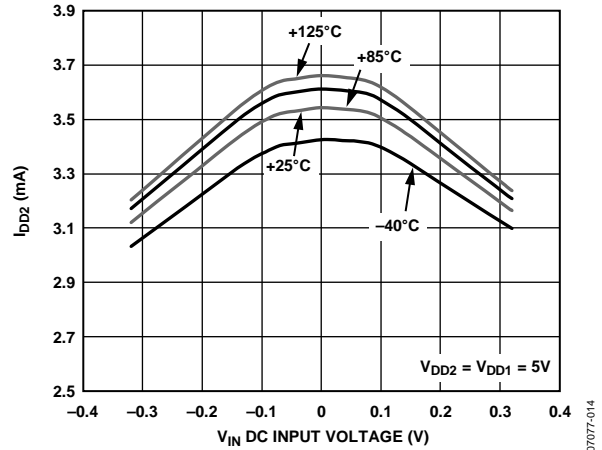
Figure 15. I_{\text{DD2}} vs. V_{\text{IN}} at Various Temperatures
