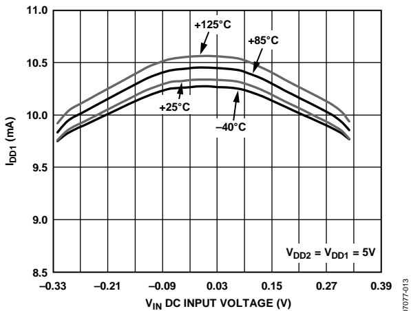
Figure 14. I_{\text{DD1}} vs. V_{\text{IN}} at Various Temperatures
