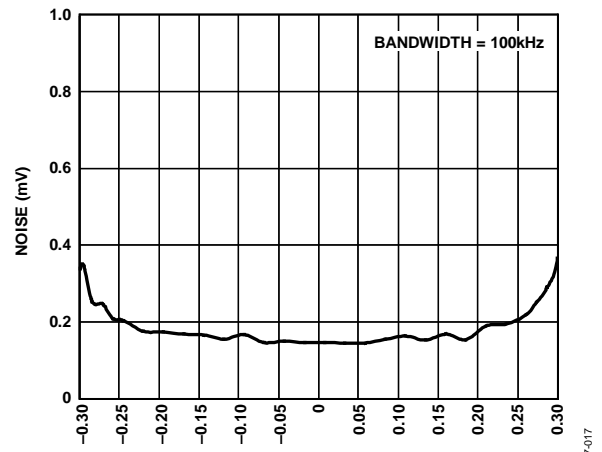
Figure 17. RMS Noise Voltage vs. V_{\text{IN}} DC Input
