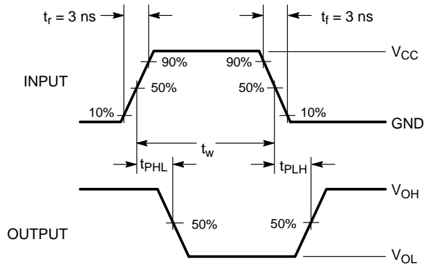
Figure 3. AC Waveforms
