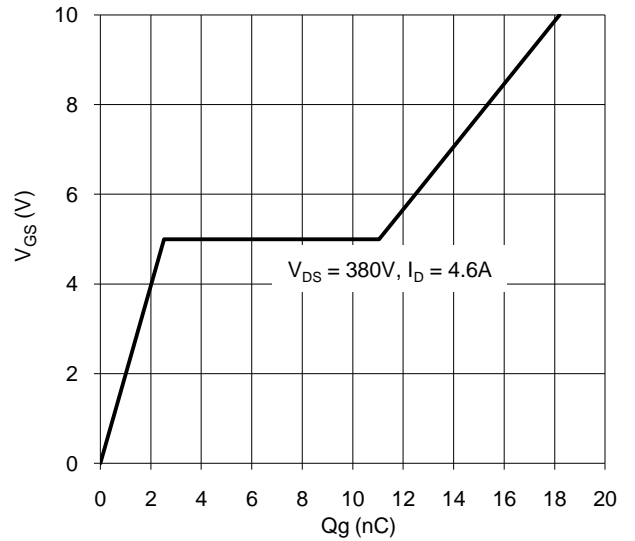
Figure 10. Gate Charge
