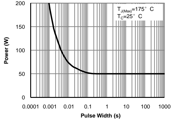
Figure 10: Single Pulse Power Rating Junction-to-Case for AOT2910L and AOB2910L (Note F)
