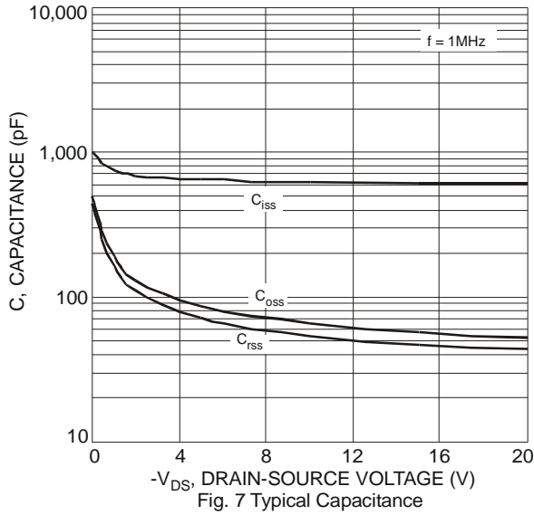
Fig. 7 Typical Capacitance
