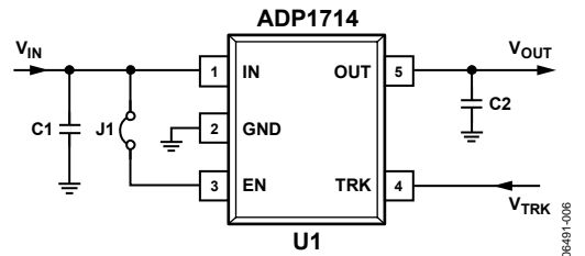
Figure 6. ADP1714 Fixed Output with Tracking
