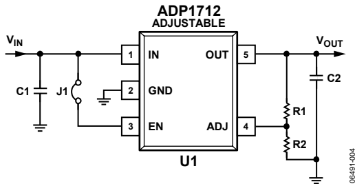
Figure 4. ADP1712 Adjustable Output
