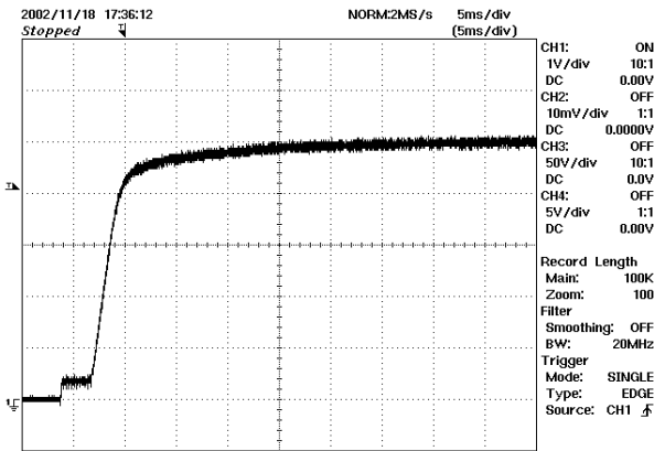
Figure 22 – Start-up Profile, 48 VDC, Full Load. 1 V/div, 5 ms/div.
