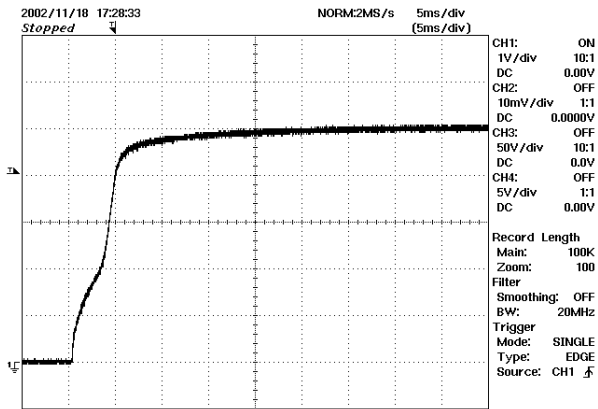
Figure 23 – Start-up Profile, 48 VDC, Zero Load. 1 V/div, 5 ms/div.
