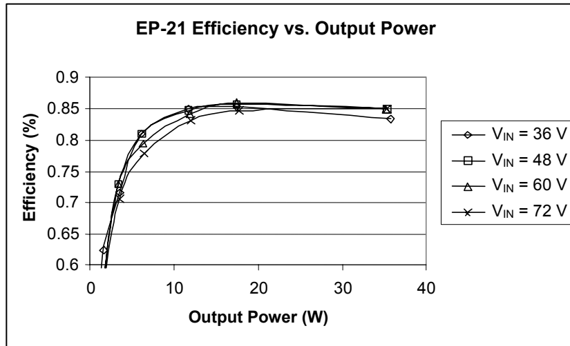
Figure 8 – Efficiency vs. Output Power, Room Temperature.
