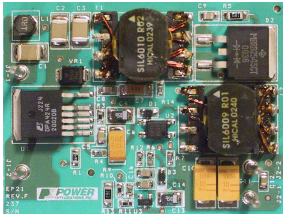
Figure 1 – EP-21 Populated Circuit Board (57.5 mm L x 43.6 mm W x 10.7 mm H).
