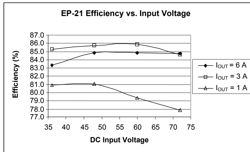
Figure 9 – Efficiency vs. Input Voltage, Room Temperature.
