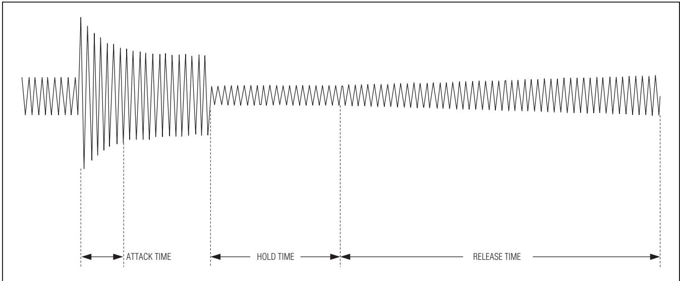
Figure 12. AGC Timing
