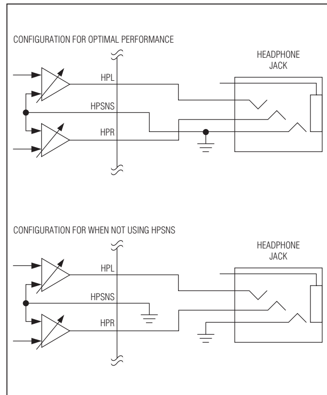
Figure 30. HPSNS configurations
