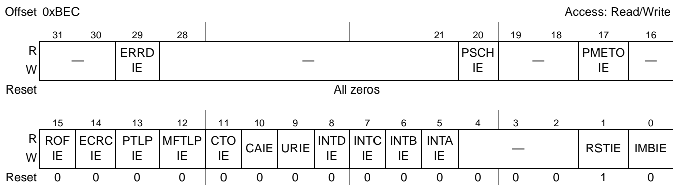
Figure 14-122. CSB System Miscellaneous Interrupt Enable Register (PEX_CSMIER)
