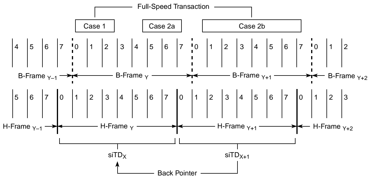
Figure 13-58. siTD Scheduling Boundary Examples
