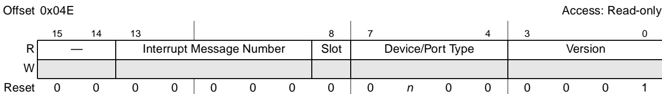
Figure 14-48. PCI Express Capabilities Register
