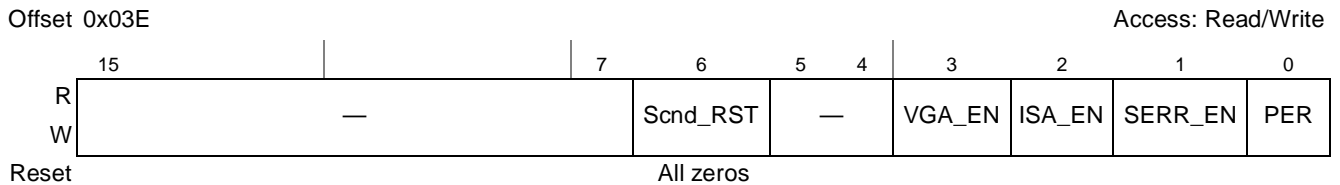
Figure 14-39. PCI Express Bridge Control Register
