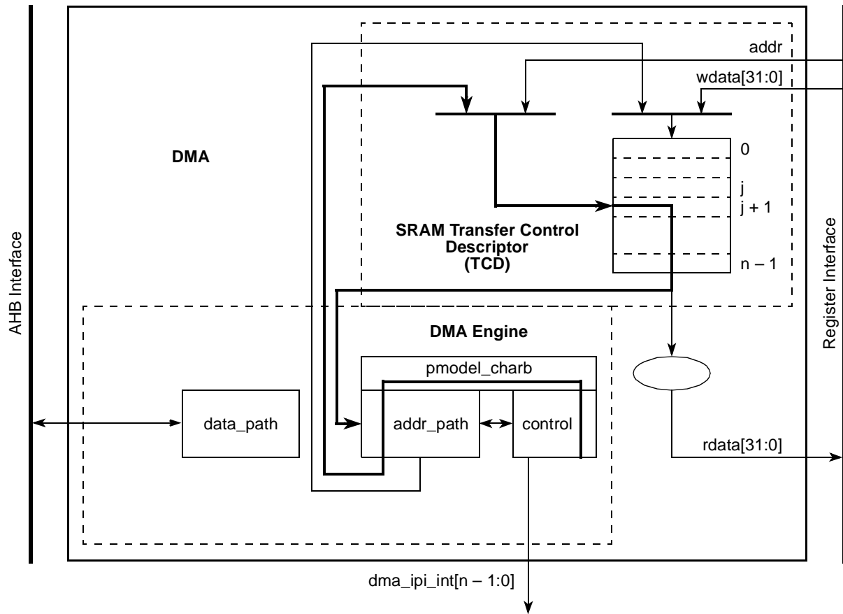
Figure 12-23. DMA Operation—Part 1
