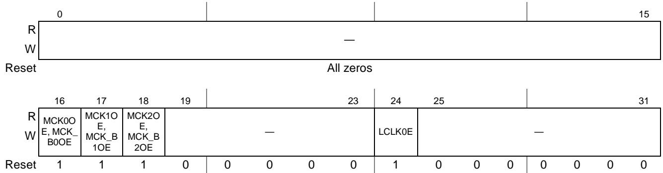
Figure 4-14. Output Clock Control Register (OCCR)
