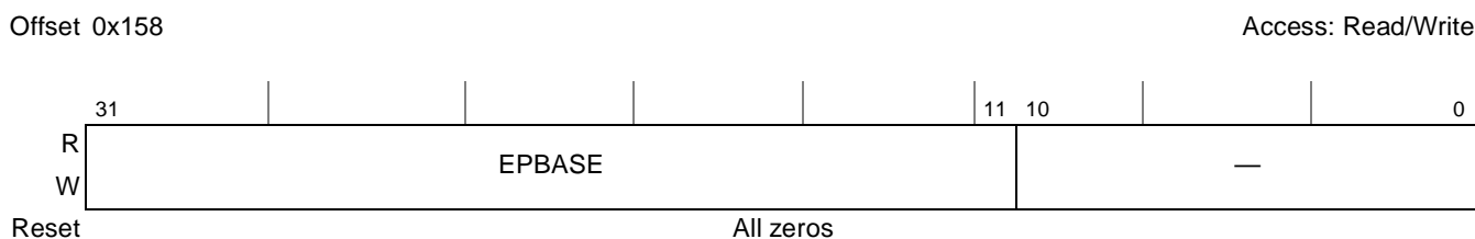
Figure 13-15. Endpoint List Address (ENDPOINTLISTADDR)
