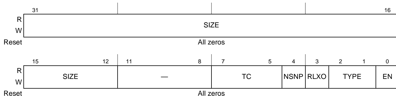
Figure 14-128. PCI Express Outbound Window Attributes Register n (PEX_OWAR0–PEX_OWAR3)
