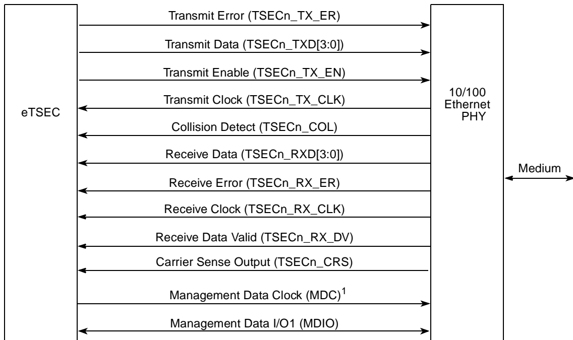
Figure 16-117. eTSEC-MII Connection
