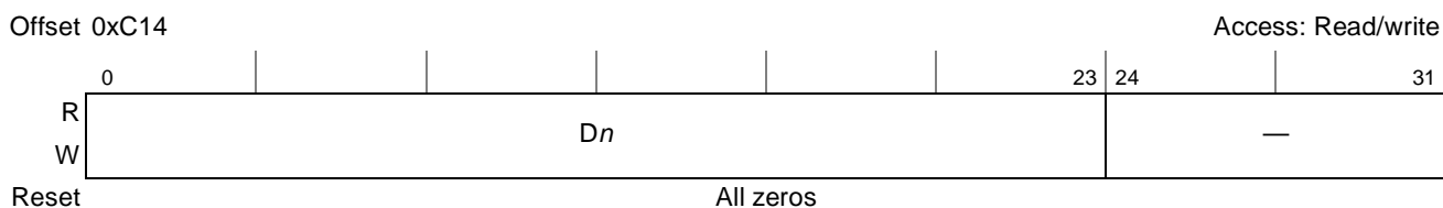
Figure 21-7. GPIO Interrupt Control Register (GPICR)
