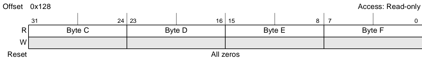
Figure 14-73. PCI Express Header Log Register
