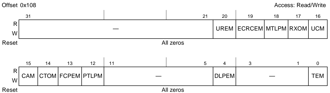
Figure 14-68. PCI Express Uncorrectable Error Mask Register
