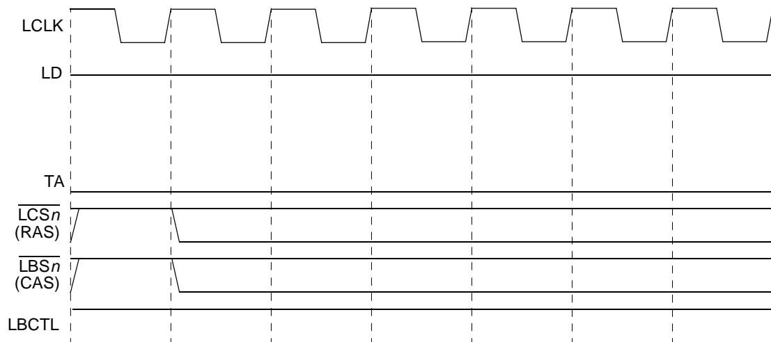
Figure 10-76. Exception Cycle
