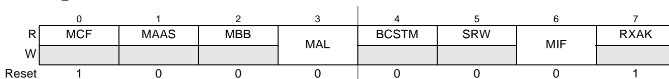
Figure 17-5. I 2 C Status Register (I2CSR)
