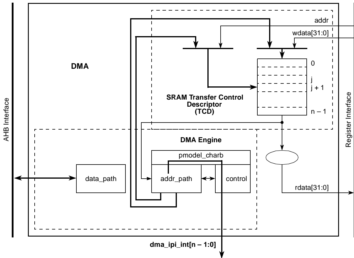
Figure 12-25. DMA Operation—Part 3
