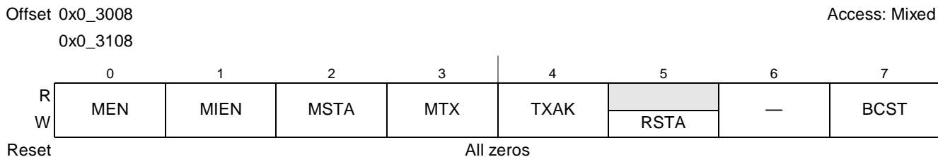
Figure 17-4. I 2 C Control Register (I2CCR)
