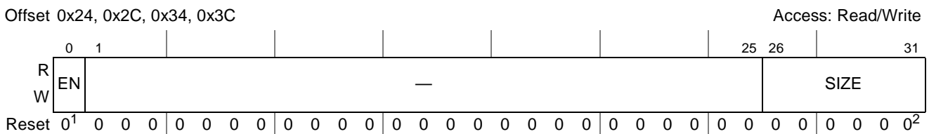
Figure 5-5. LBC Local Access Window n Attributes Registers (LBLAWAR0–LBLAWAR3)
