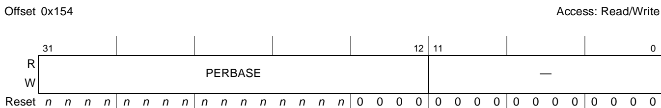
Figure 13-12. Periodic Frame List Base Address (PERIODICLISTBASE)
