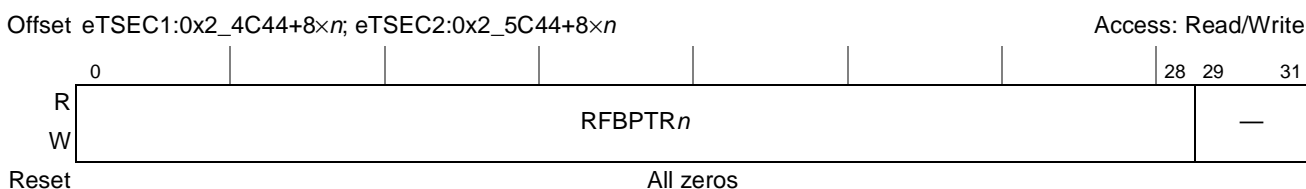
Figure 16-104. RFBPTR0–RFBPTR7 Register Definition
