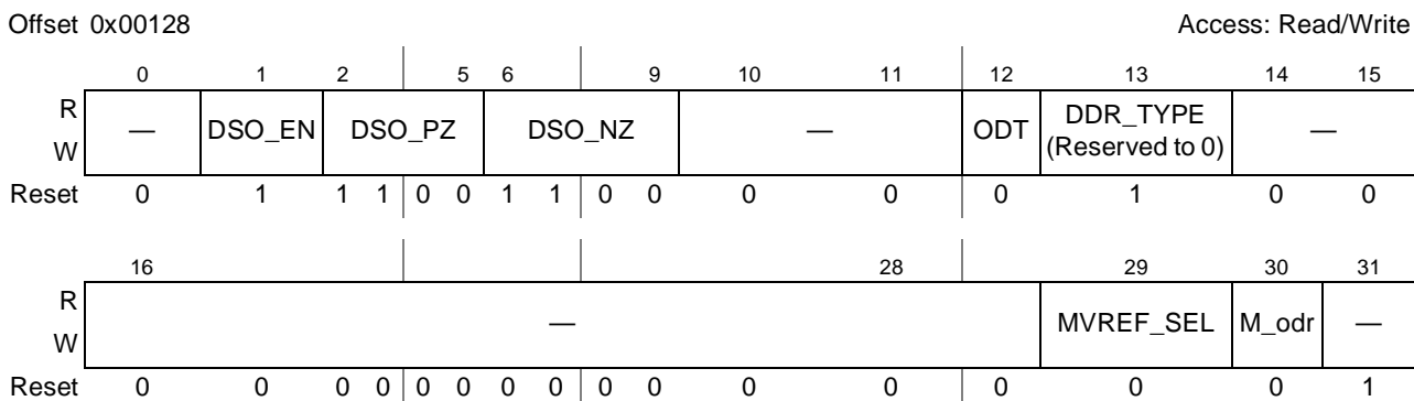
Figure 5-16. DDR Control Driver Register (DDRCDR)
