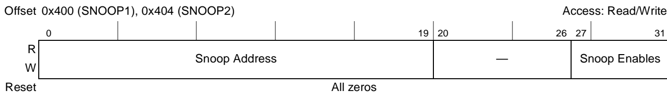
Figure 13-30. Snoop 1 and Snoop 2 (SNOOP n )
