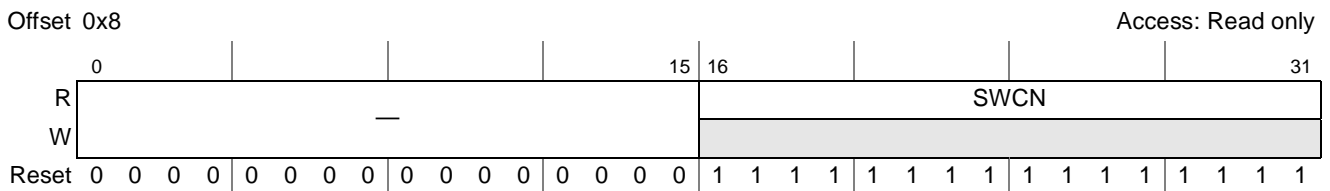
Figure 5-23. System Watchdog Count Register (SWCNR)
