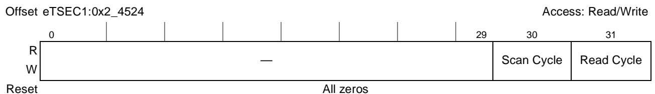
Figure 16-41. MIIMCOM Register Definition
