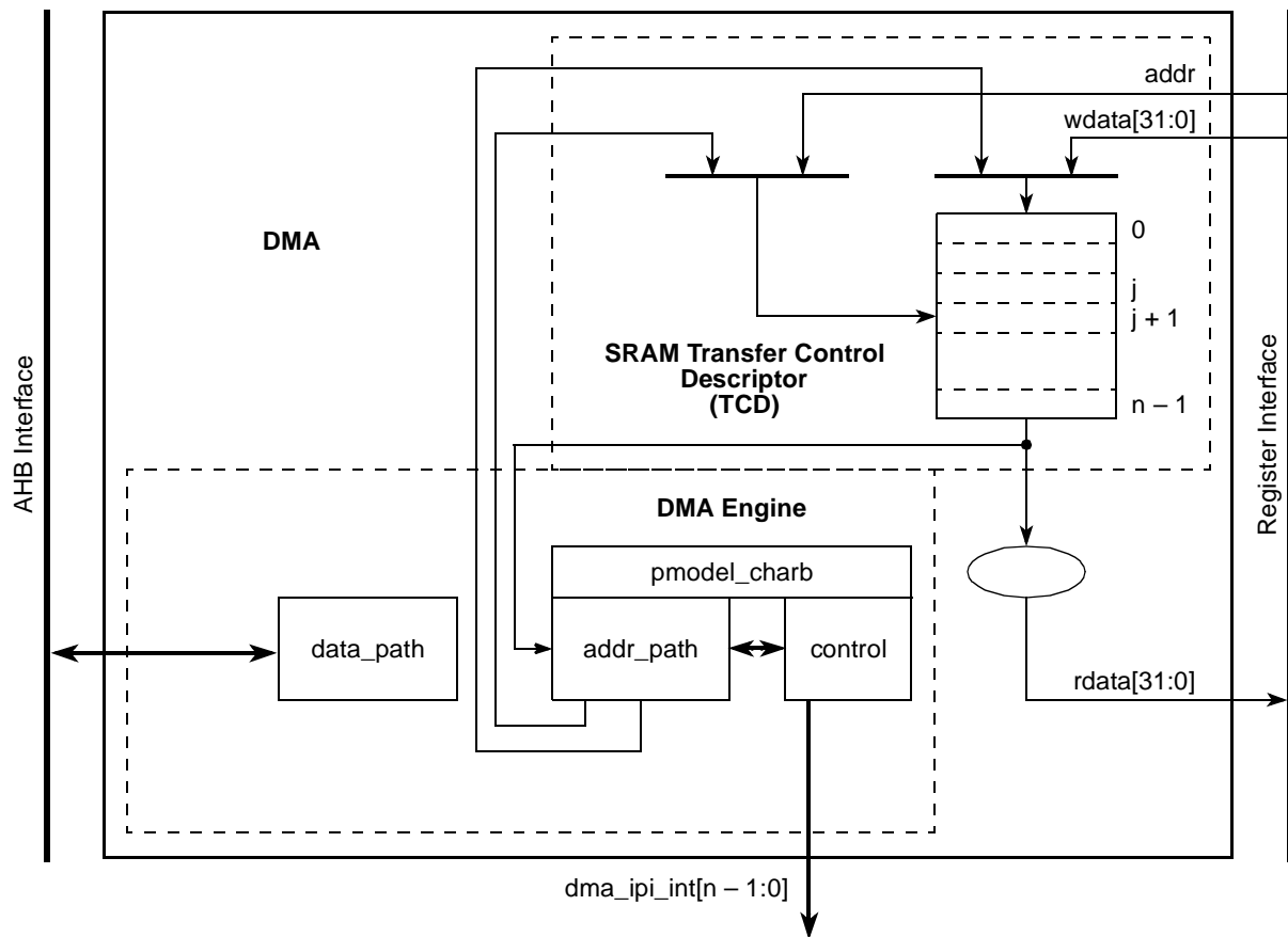
Figure 12-24. DMA Operation—Part 2
