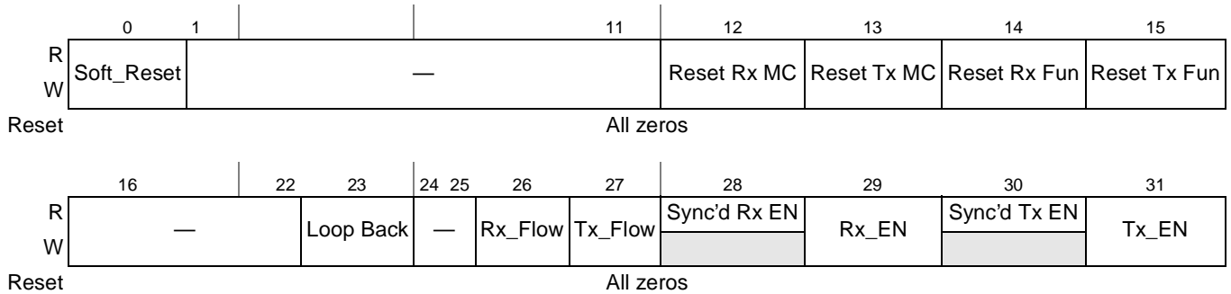
Figure 16-35. MACCFG1 Register Definition
