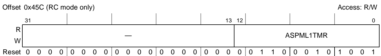
Figure 14-83. PCI Express ASPM Request Timer Register
