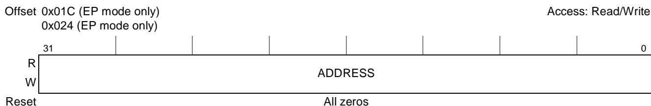
Figure 14-15. 64-Bit High Memory Base Address Registers 3 and 5 (BAR3/BAR5)
