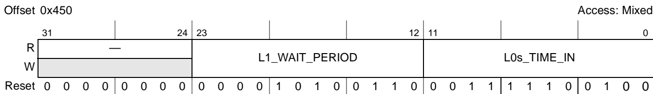
Figure 14-81. PCI Express Power Management Timer Register (PEX_PM_TIMER)
