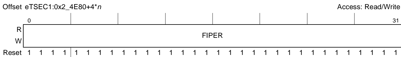
Figure 16-115. TMR_FIPERn Register Definition
