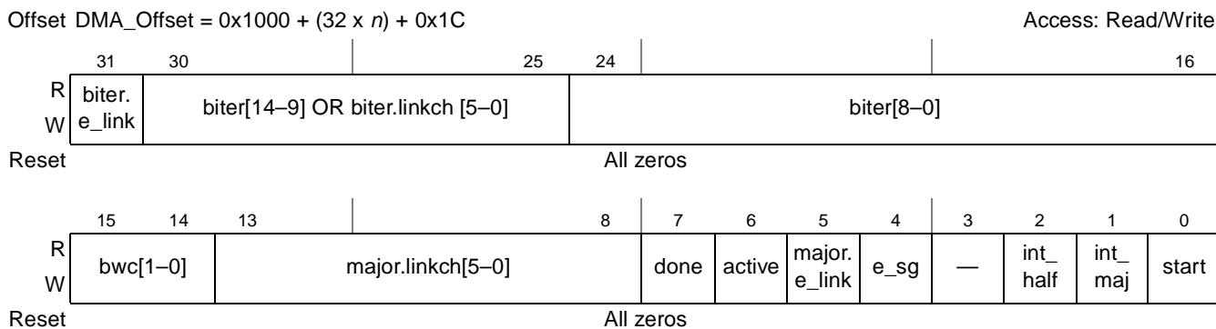
Figure 12-22. TCD Word 7 (TCDn.{biter, control/status}) Fields
