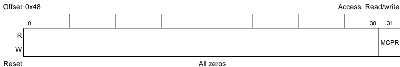
Figure 8-20. System Error Control Register (SERCR)
