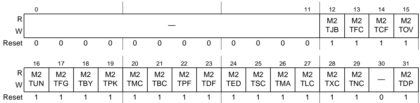
Figure 16-97. Carry Mask Register 2 (CAM2) Register Definition
