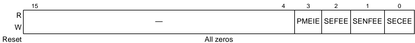
Figure 14-58. PCI Express Root Control Register
