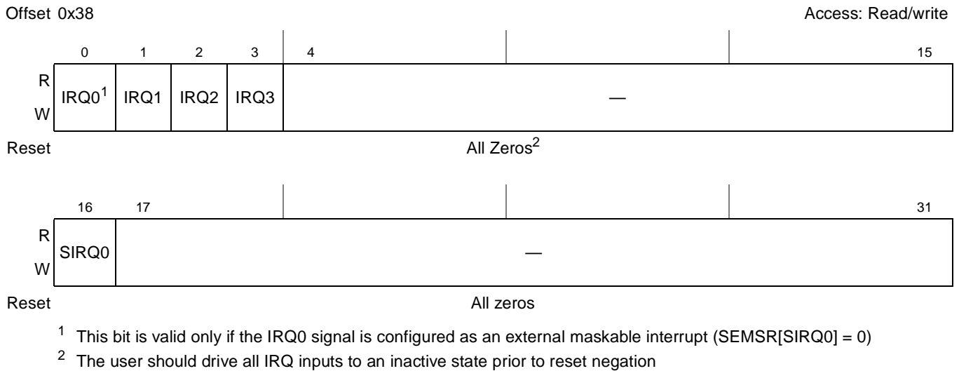
Figure 8-16. System External Interrupt Mask Register (SEMSR)
