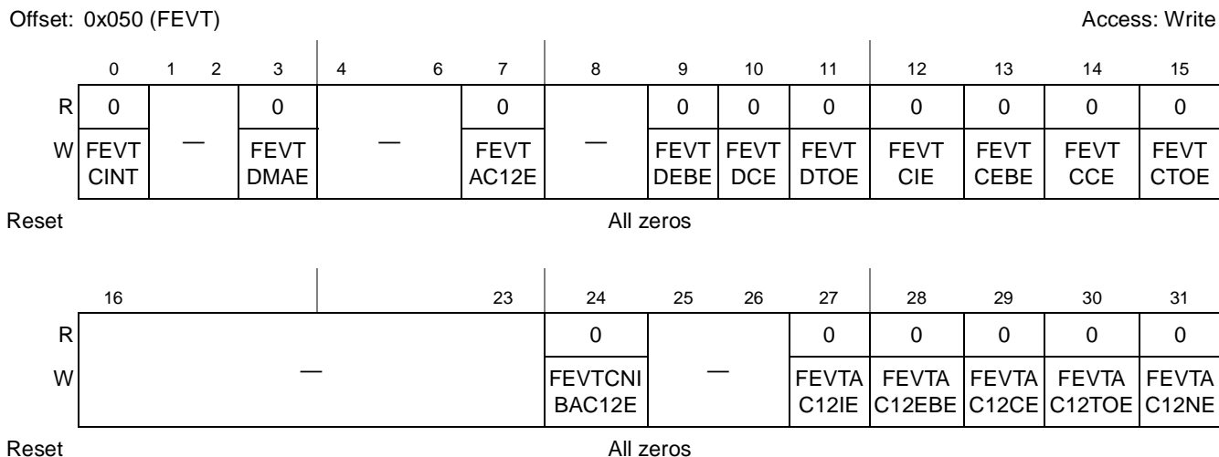
Figure 11-18. Force Event Register (FEVT)
