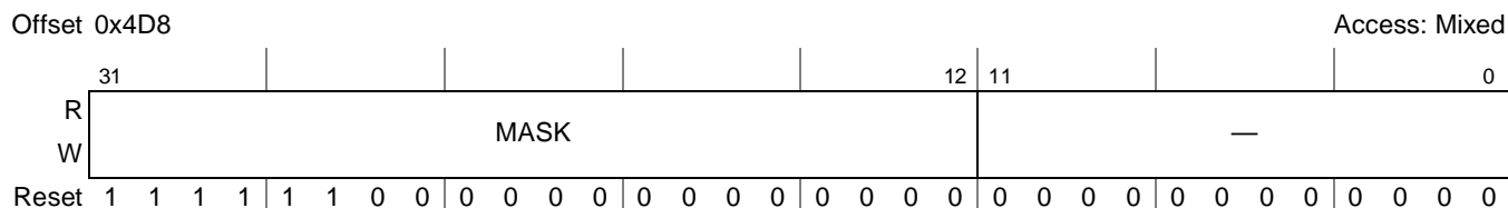
Figure 14-89. PCI Express BAR Size Low Configuration Register (PEX_BAR_SIZEL)
