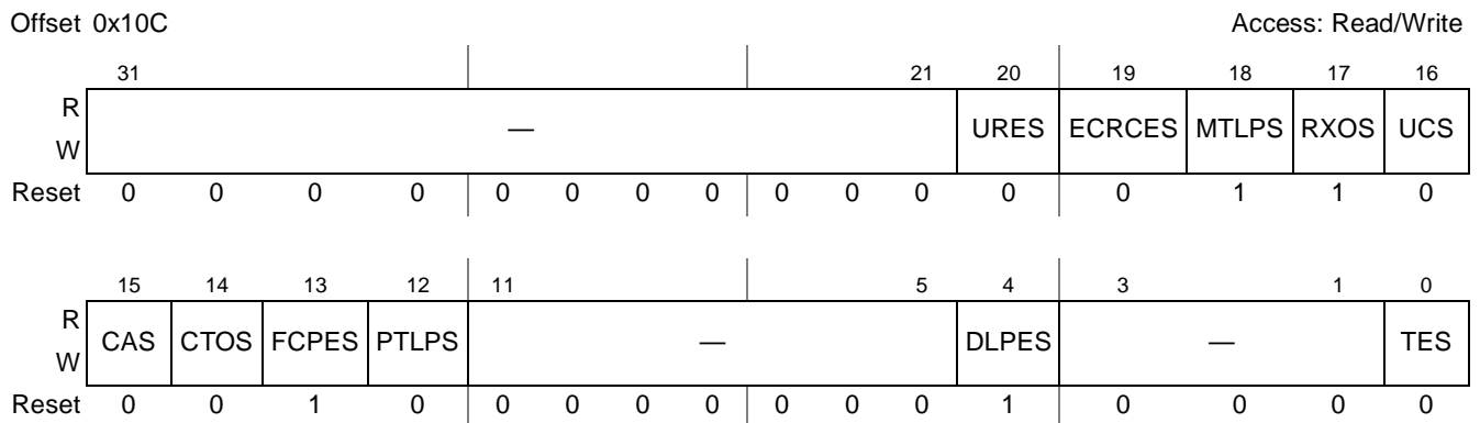
Figure 14-69. PCI Express Uncorrectable Error Severity Register
