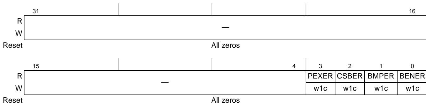
Figure 14-99. PCI Express Outbound PIO Status Register (PEX_CSB_OBSTAT)
