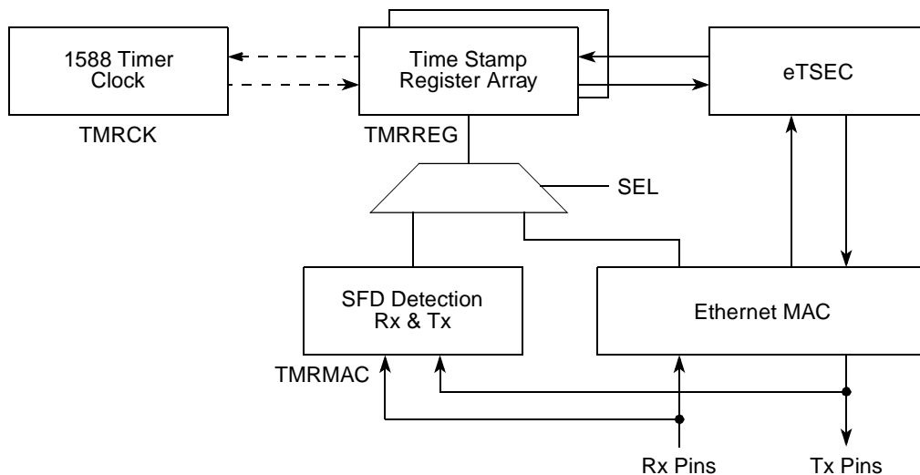
Figure 16-126. 1588 Timer Design Partition
