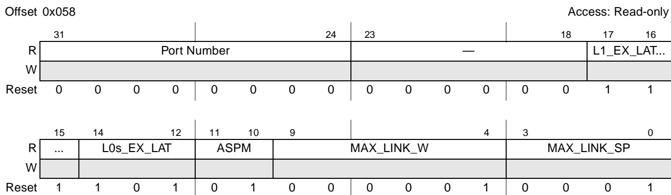
Figure 14-52. PCI Express Link Capabilities Register
