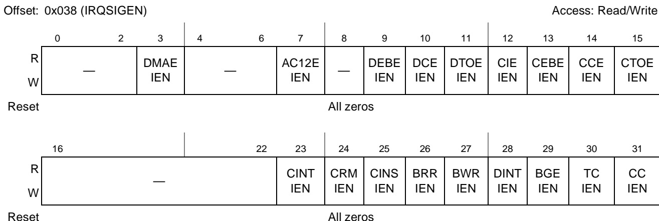
Figure 11-14. Interrupt Signal Enable Register (IRQSIGEN)
