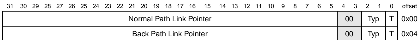
Figure 13-42. Frame Span Traversal Node Structure
