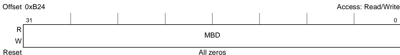
Figure 14-109. MPCl Express Outbound Mailbox Data Register (PEX_OMBDR)
