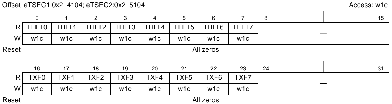
Figure 16-12. TSTAT Register Definition
