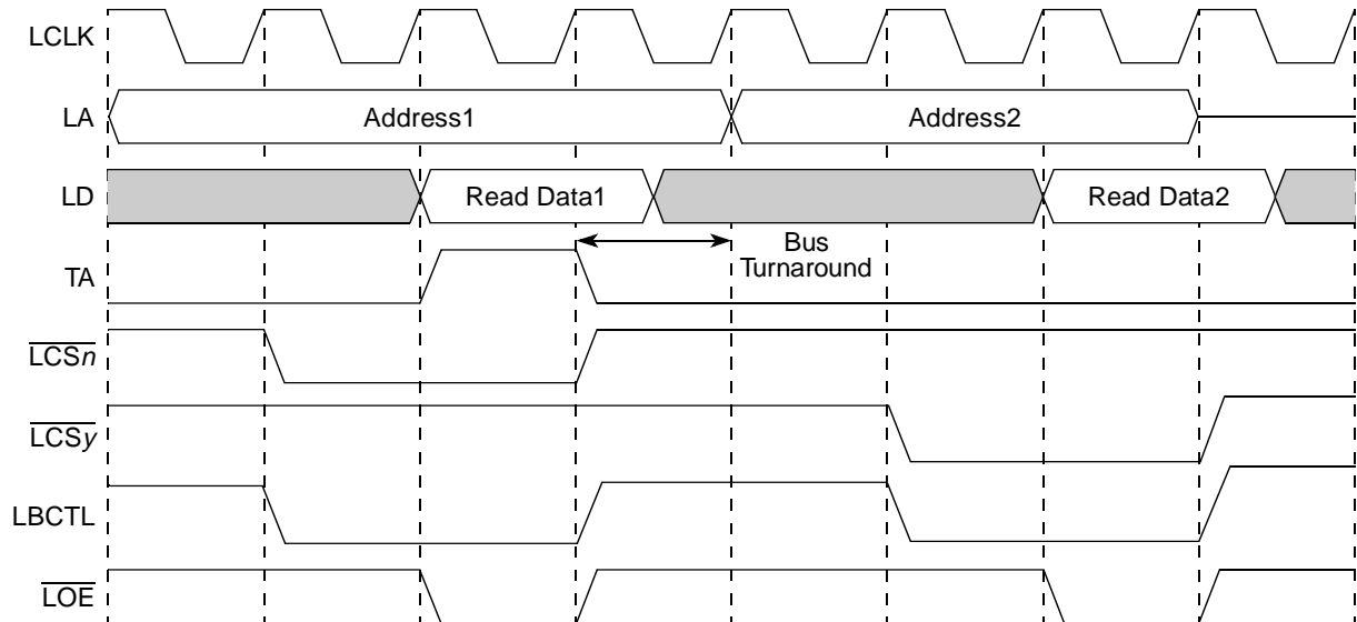
Figure 10-41. GPCM Read Followed by Read ( \text{TRLX} = 0 , \text{EHTR} = 0 , Fastest Timing)
