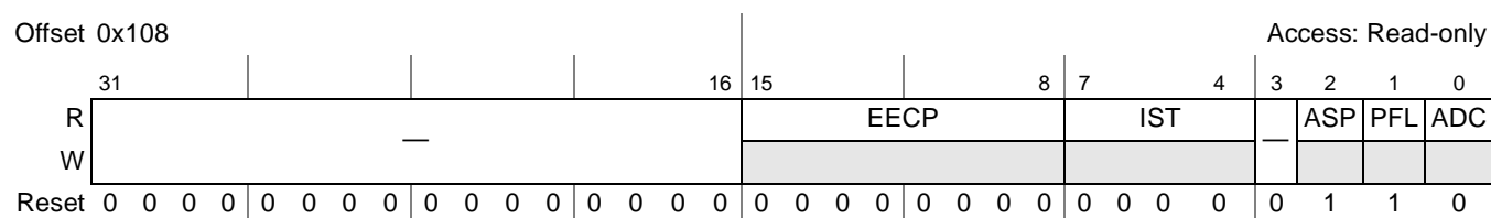
Figure 13-5. Host Control Capability Parameters (HCCPARAMS)
