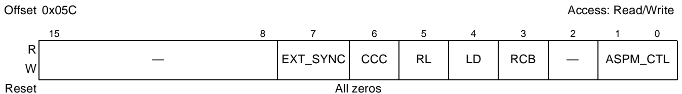
Figure 14-53. PCI Express Link Control Register
