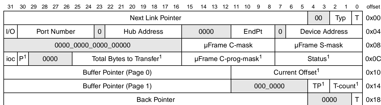
Figure 13-39. Split-Transaction Isochronous Transaction Descriptor (siTD)
