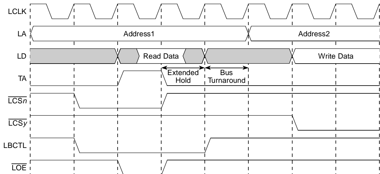
Figure 10-42. GPCM Read Followed by Write ( \text{TRLX} = 0 , \text{EHTR} = 1 , One-Cycle Extended Hold Time on Reads)
