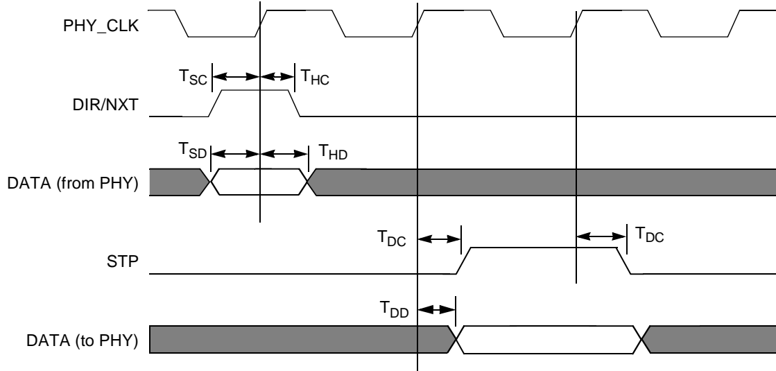
Figure 13-66. ULPI Timing
