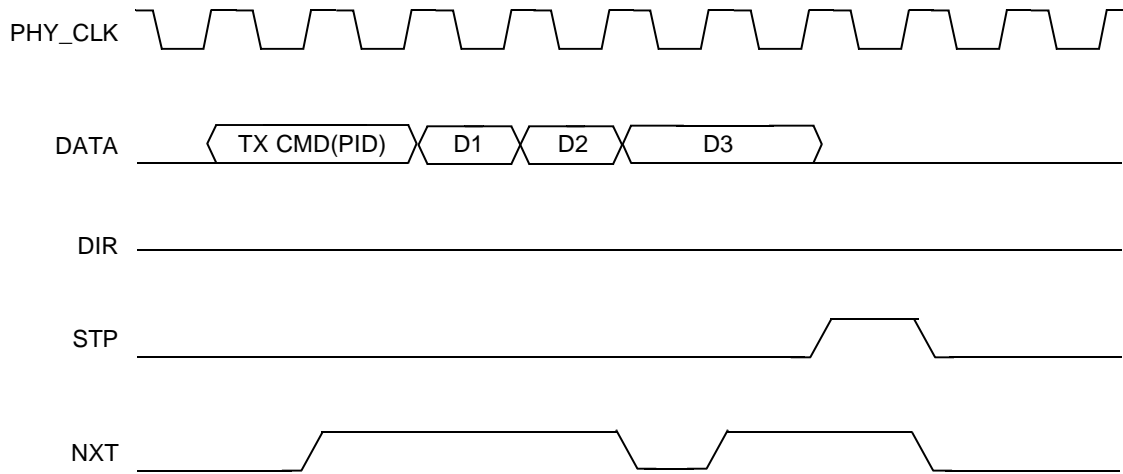
Figure 13-69. ULPI Data Transmit (PID)
