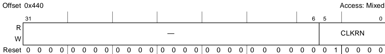
Figure 14-80. PCI Express Core Clock Ratio Register (PEX_GCLK_RATIO)
