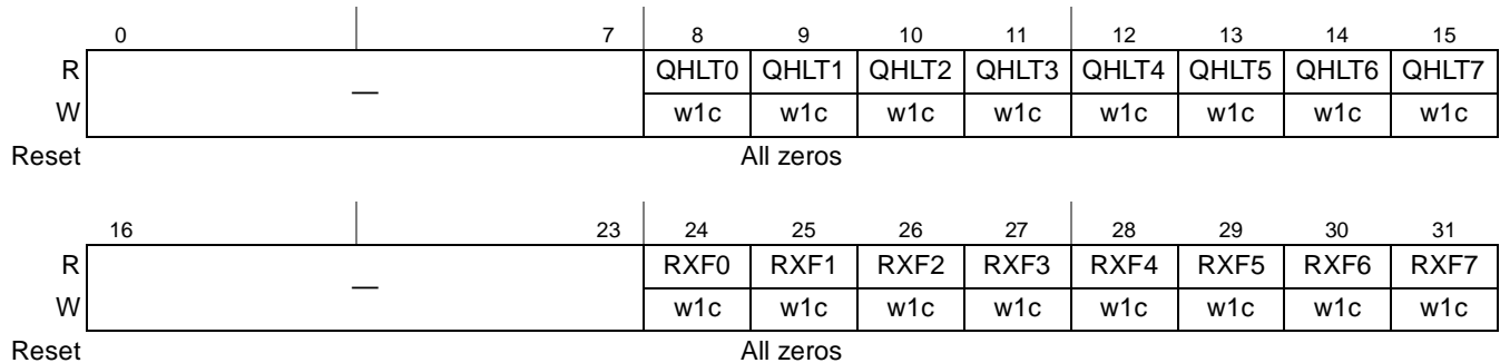
Figure 16-23. RSTAT Register Definition
