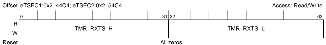
Figure 16-34. TMR_RXTS_H/L Register Definition
