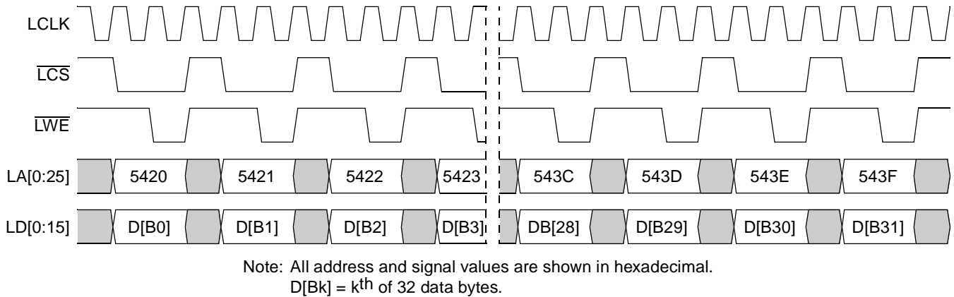
Figure 10-30. Example of 8-Bit GPCM Writing 32 Bytes to Address 0x5420 (LCRR[PBYP] = 0)
