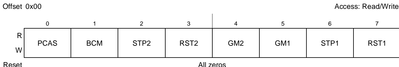
Figure 5-43. Global Timers Configuration Register 1 (GTCFR1)
