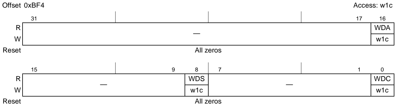
Figure 14-124. CSB System Write DMA Interrupt Status Register (PEX_CSWDISR)
