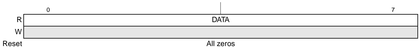
Figure 18-2. Receiver Buffer Registers (URBR1 and URBR2)
