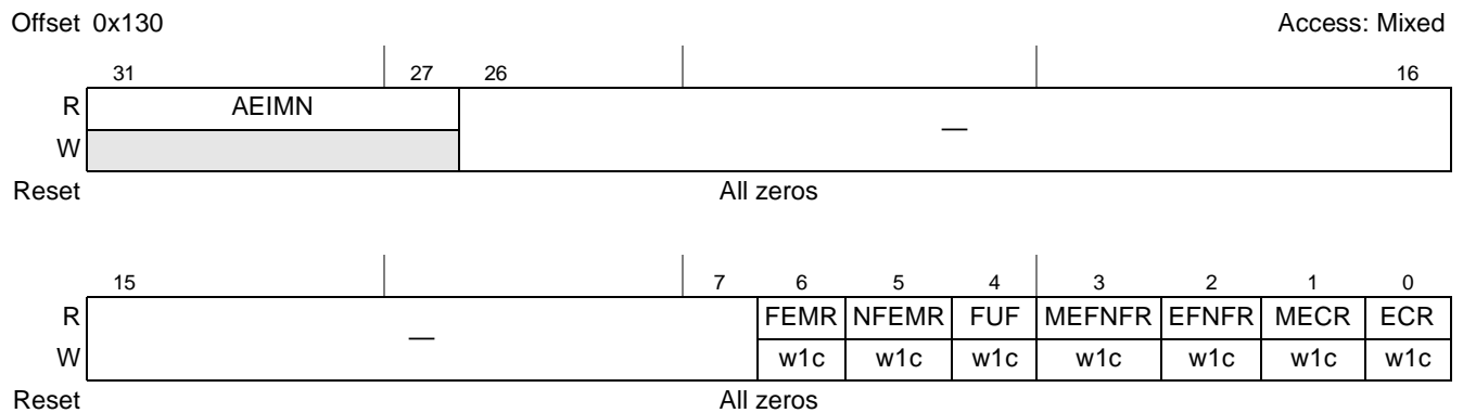
Figure 14-75. PCI Express Root Error Status Register
