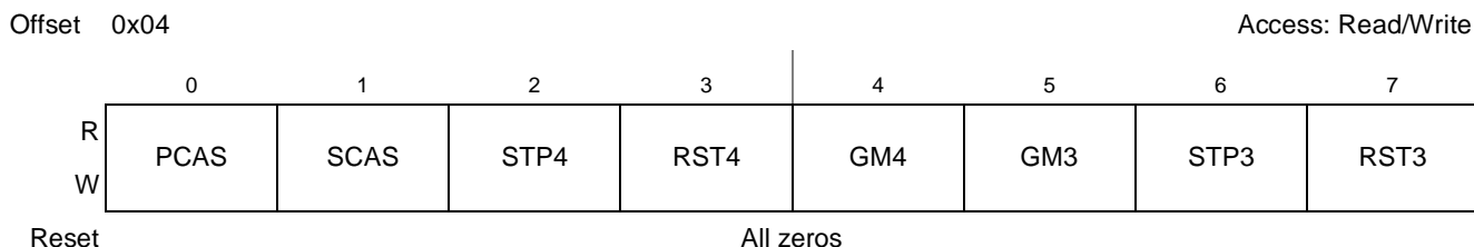
Figure 5-44. Global Timers Configuration Register 2 (GTCFR2)
