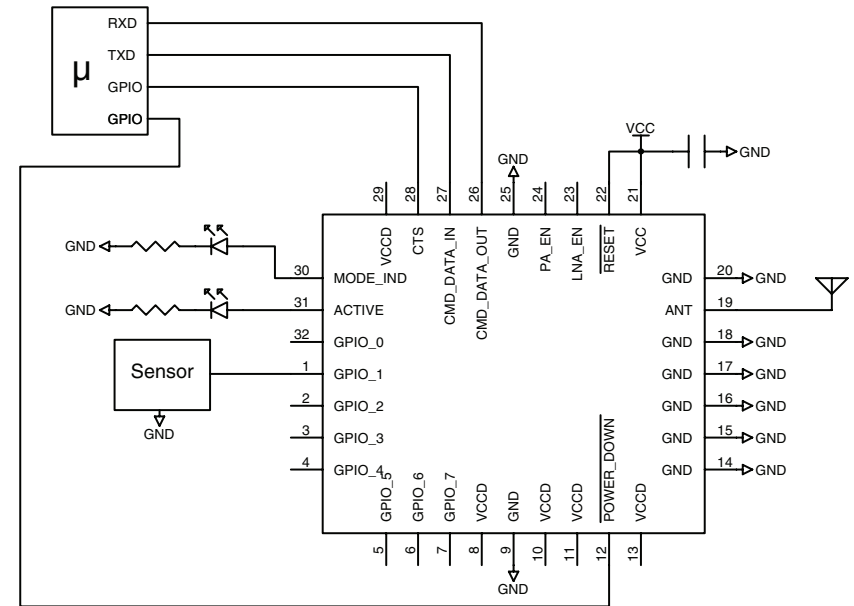
Figure 59: HumDT™ Series Transceiver Basic Application Circuit
