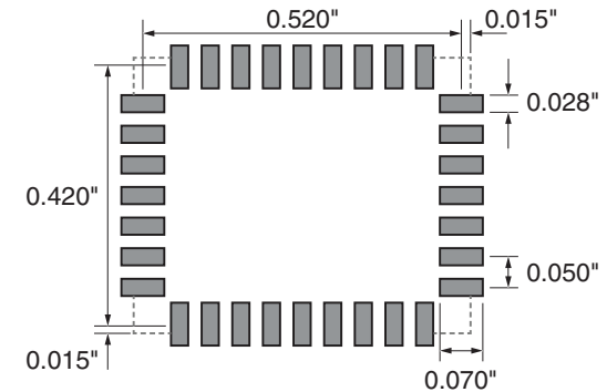
Figure 63: Recommended PCB Layout
