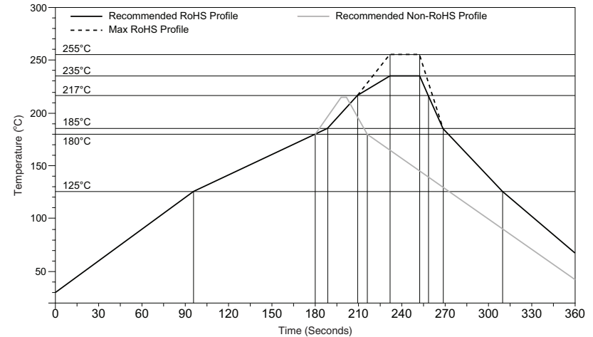
Figure 68: Maximum Reflow Temperature Profile
