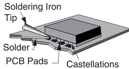
Figure 66: Soldering Technique
