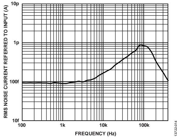
Figure 10. Noise Bandwidth/Peaking
