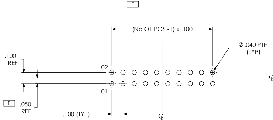
FIG 2 -RA AND -TH OPTION
