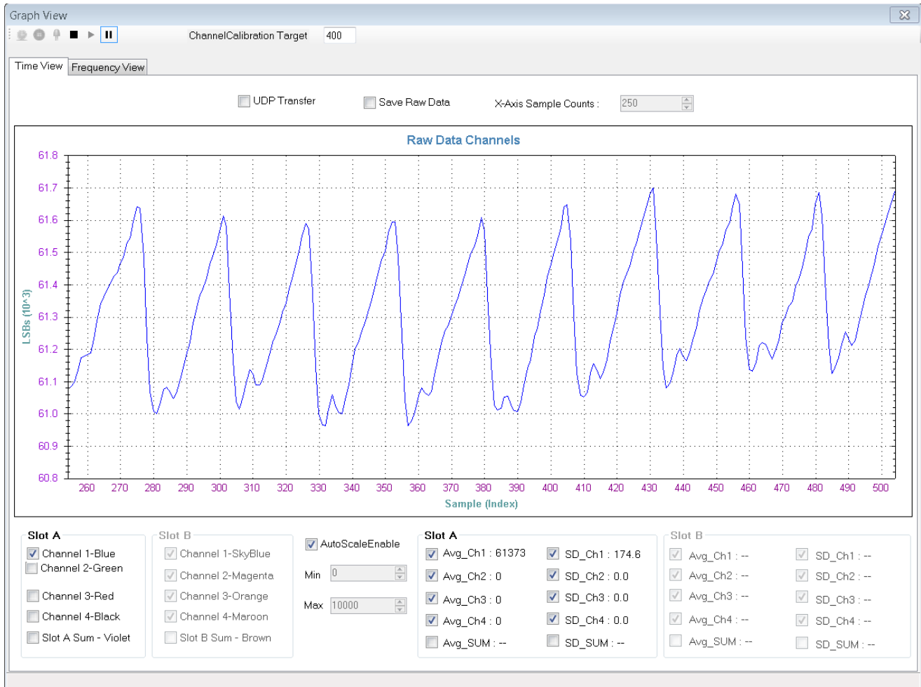
Figure 24. Time View
