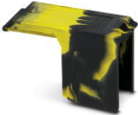
Covering hood, length: 164 mm, width: 49 mm, height: 33 mm, color: black/yellow
