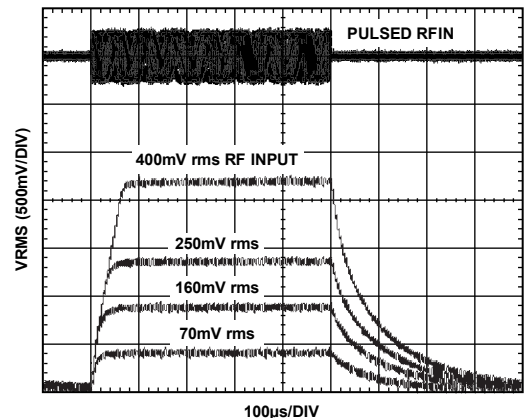
Figure 33. Output Response to Various RF Input Pulse Levels, Supply = 3 V, Frequency = 900 MHz, C_{FLTR} = \text{Open} , C_{OUT} = 0.1\text{ µF} , R_{OUT} = 1\text{ k}\Omega
