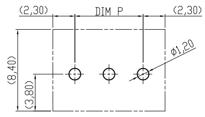
RECOMMENDER PCB LAYOUT
