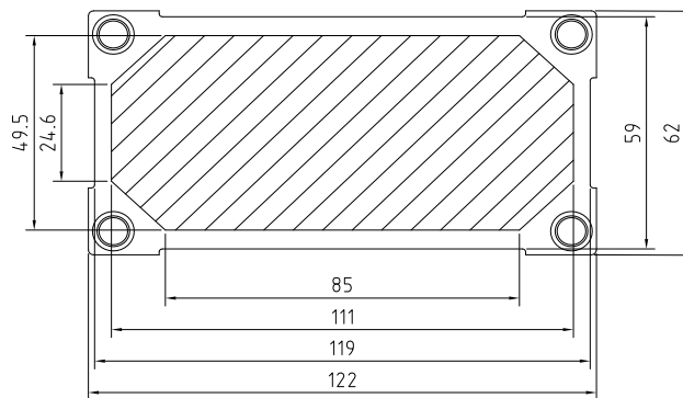
restricted area for Thermal Interface Material
