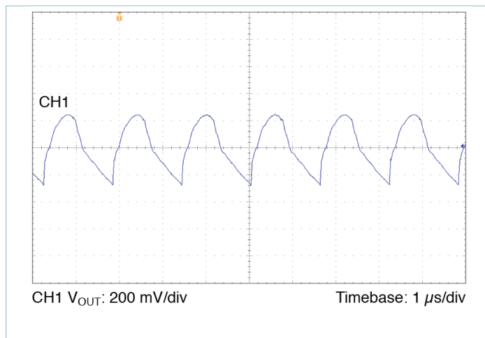
Figure 19 — Output voltage ripple, V_{IN} = 24\text{ V} , V_{OUT} = 12.0\text{ V} , C_{OUT\_EXT} = 1000\ \mu\text{F} , R_{LOAD} = 0.450\ \Omega
