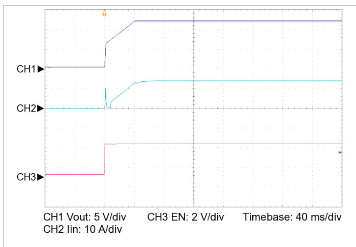
Figure 17 — Startup from EN, V_{IN} = 24\text{ V} , C_{OUT\_EXT} = 10000\ \mu\text{F} , R_{LOAD} = 0.450\ \Omega
