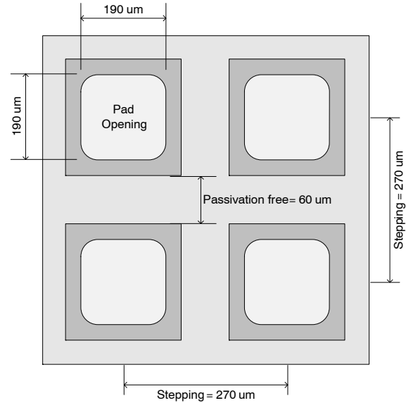
Figure 1. Wafer Array
