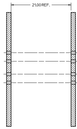
SECTION Z-Z
