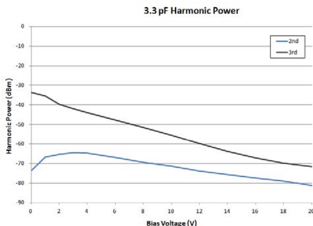
Figure 3. Harmonic Power
