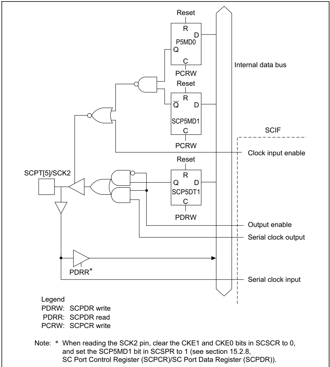
Figure 17.2 SCPT[5]/SCK2 Pin
