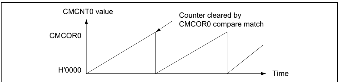
Figure 12.27 Counter Operation
