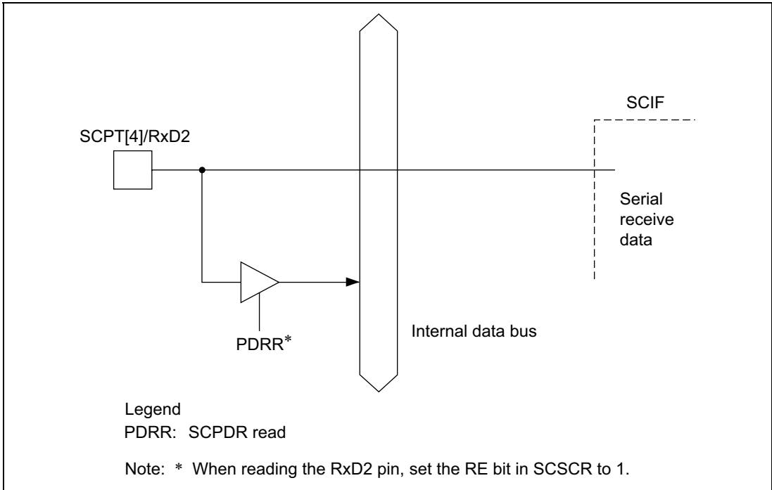
Figure 17.4 SCPT[4]/RxD2 Pin
