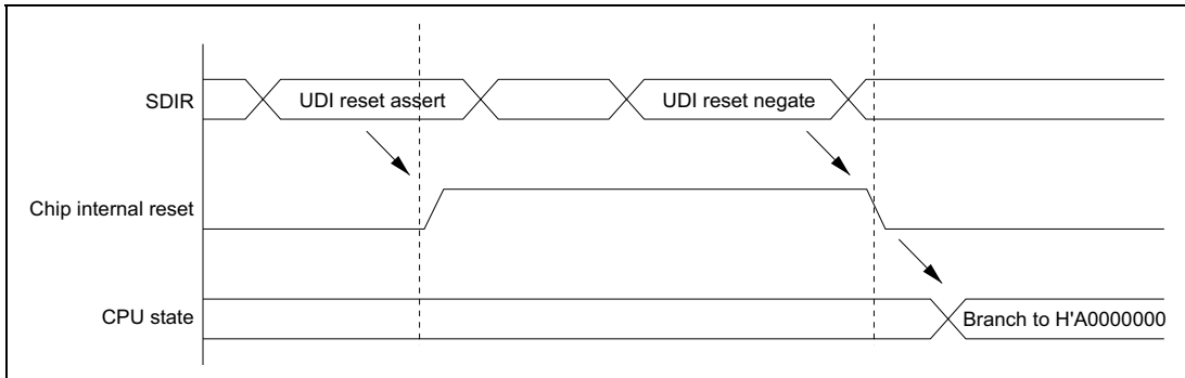
Figure 23.3 UDI Reset
