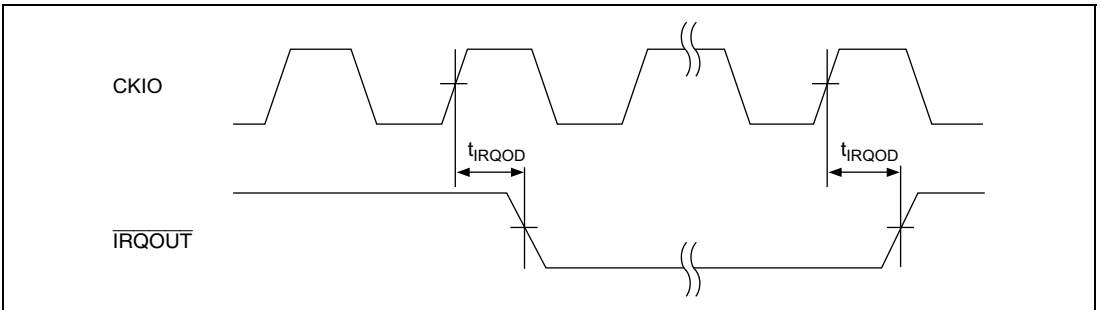
Figure 24.13 \overline{IRQOUT} Timing
