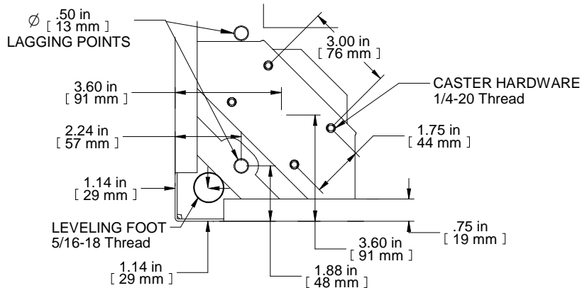
DETAIL A 4X SCALE 5:1
