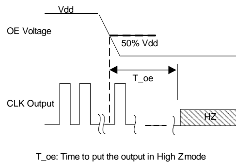
Figure 7. OE Disable Timing (OE Mode Only)
