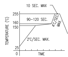
C LEAD FREE REFLOW PROFILE
