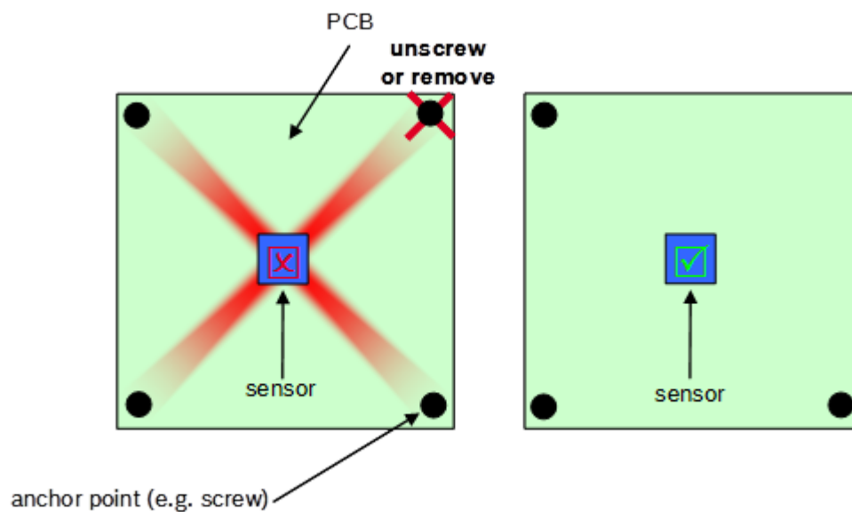
Figure 2: redundant PCB anchor points
