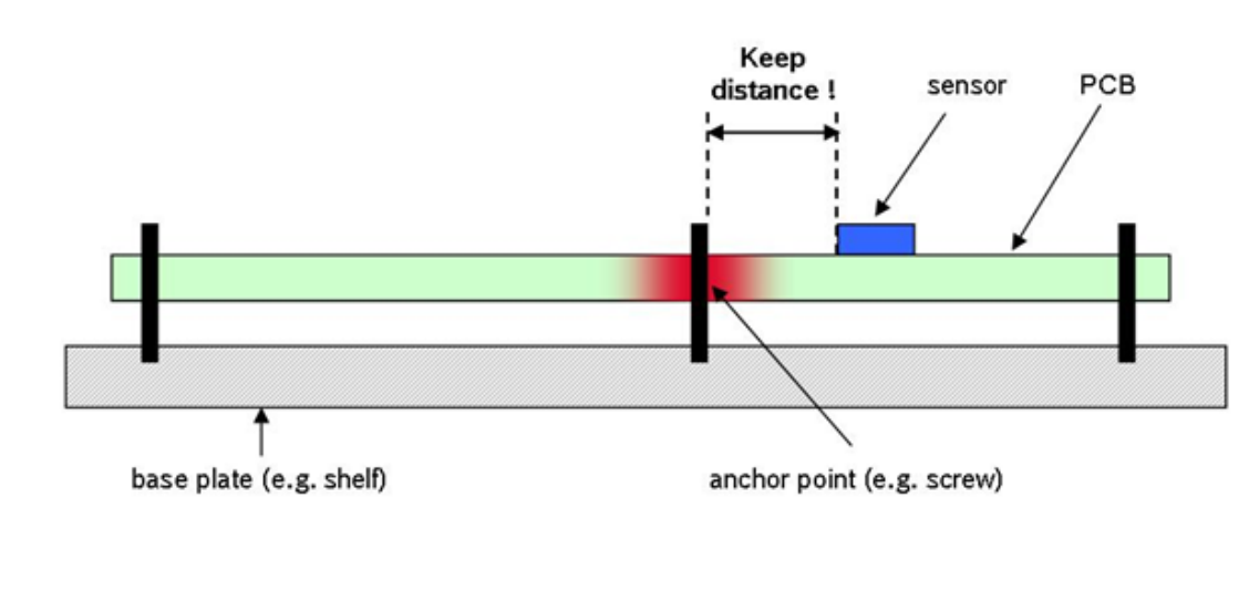
Figure 4: Distance to PCB anchor points
