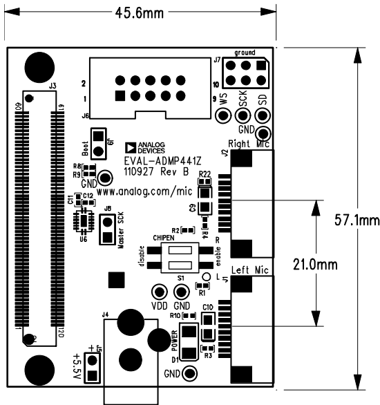
Figure 2. Evaluation Board Dimensions shown in millimeters
