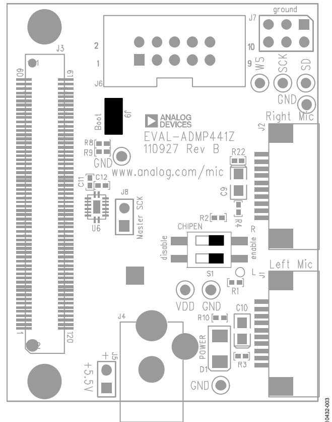
Figure 3. Top View of EVAL-ADMP441Z Board with Default Switch and Jumper Settings
