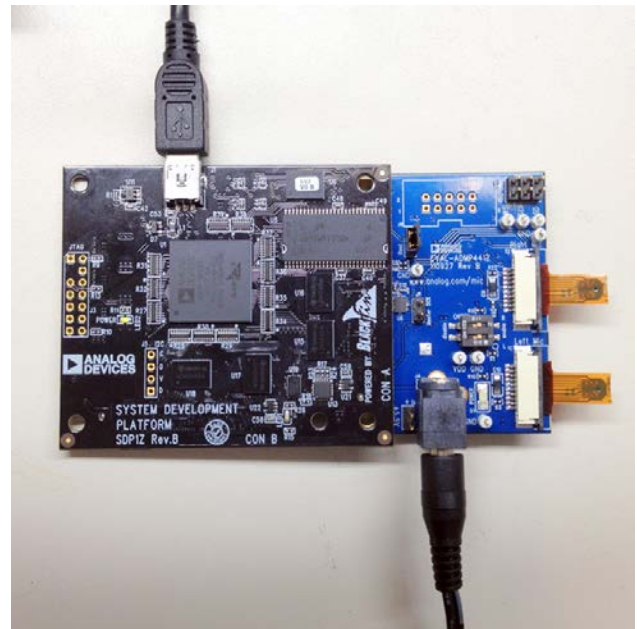
Figure 4. EVAL-ADMP441Z with Two Flex Boards Connected to an SDP-B Controller Board
