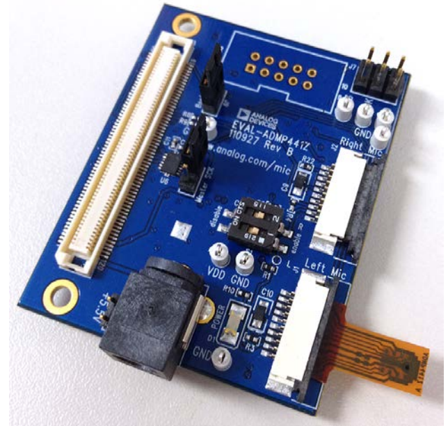
Figure 1. Evaluation Board Photo
