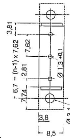
Pin layout
