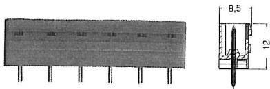
Pin layout
