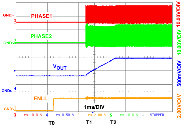
FIGURE 6. ISL6310EVAL1Z START-UP INTO A PARTIALLY CHARGED OUTPUT ( V_{DAC} = 1.200V )
