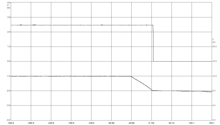
Top Trace: Output Voltage (1.0 V / div) Time Scale: (20 ms / div) Bottom Trace: Input Voltage (4 V / div)
