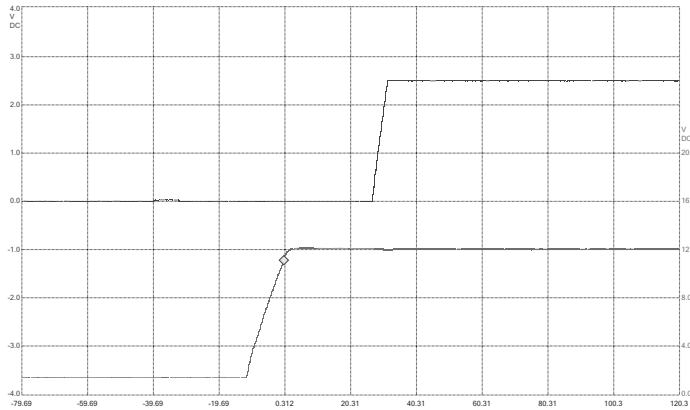
Top Trace: Output Voltage (1.0 V / div) Time Scale: (20 ms / div) Bottom Trace: Input Voltage (4 V / div)
