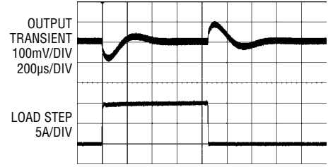
5V Transient Response
