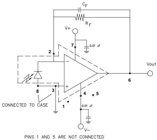
PHOTOVOLTAIC MODE
