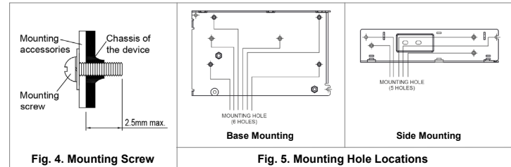
Fig. 4. Mounting Screw
