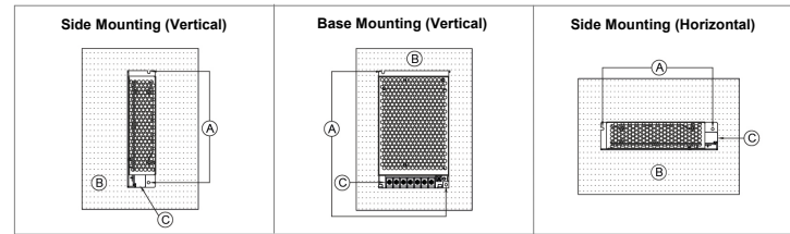
Fig. 2. Mounting Orientation
